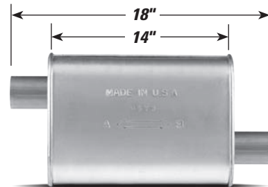
OFFSET/OFFSET (4 1/4" x 8 3/4")
