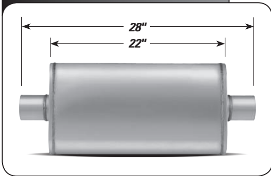
CENTER/CENTER (5" x 11")
