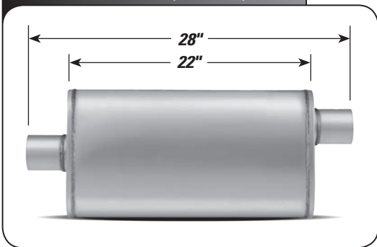
CENTER/OFFSET (5" x 11")
