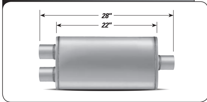
DUALS/CENTER
