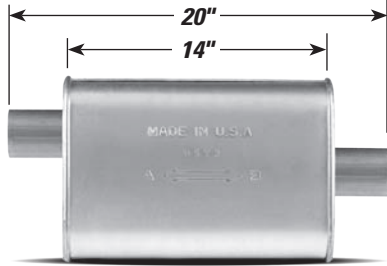
OFFSET/CENTER (3 1/4" x 7 3/4")
