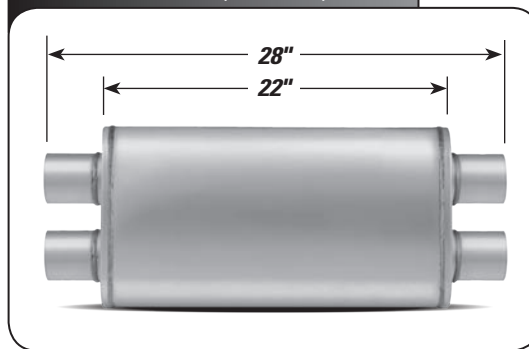
DUALS/DUALS (5" x 11")
