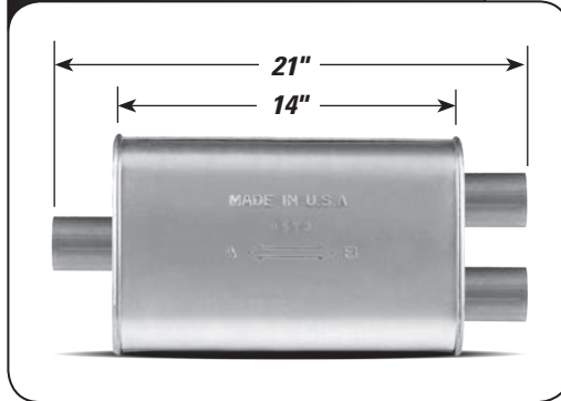
CENTER/DUALS (4 1/16" x 10 1/2")
